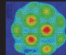
Spin-Drive pimple • A more homogeneous contact area • better contact with the ball • Less overpressure
