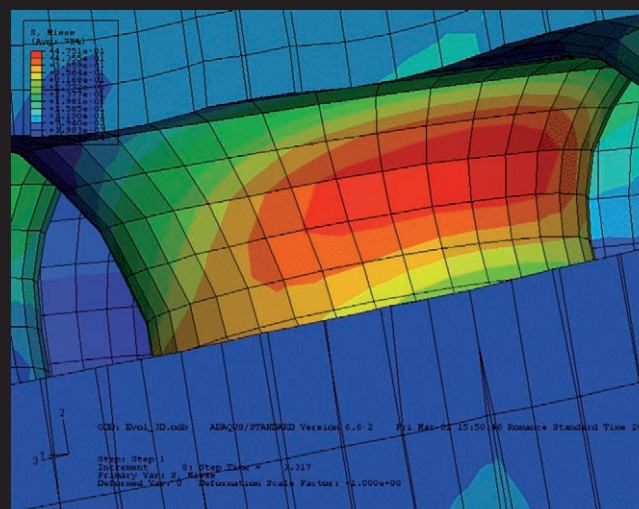
Spin-Drive pimple
