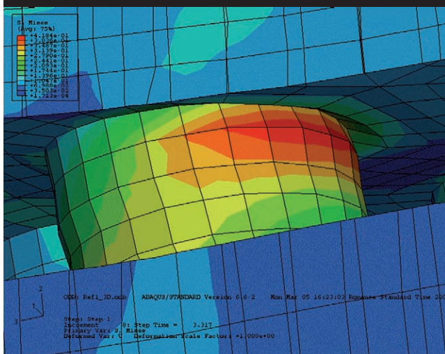
Traditional pimple
