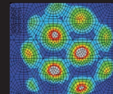
Traditional pimple • Numerous non contact areas with the ball • Important zones of Overpressure
